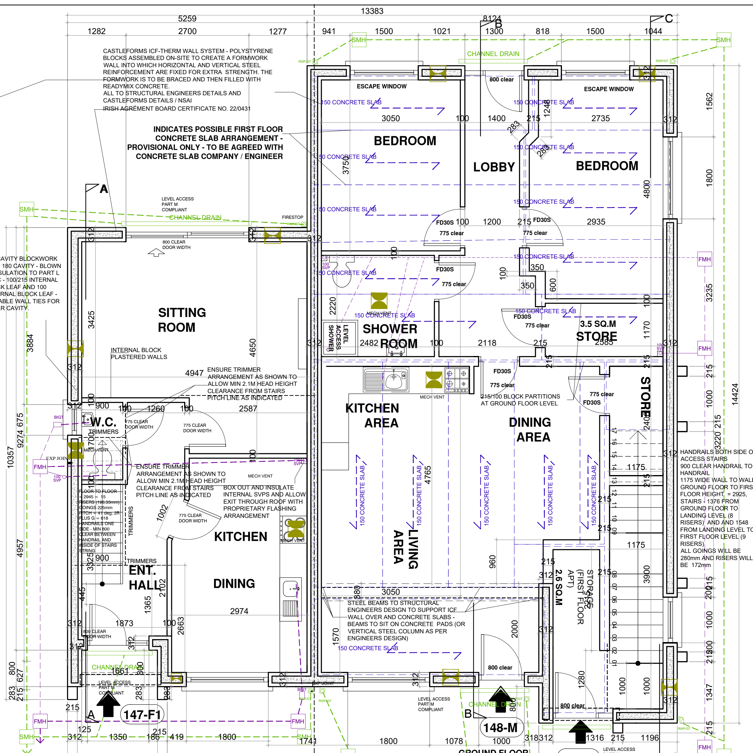
DWELLING AREA = 92 SQ.M
