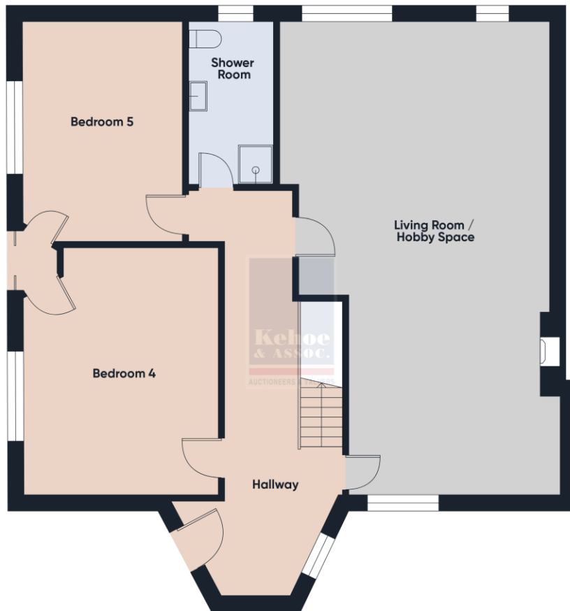
Floor 0
