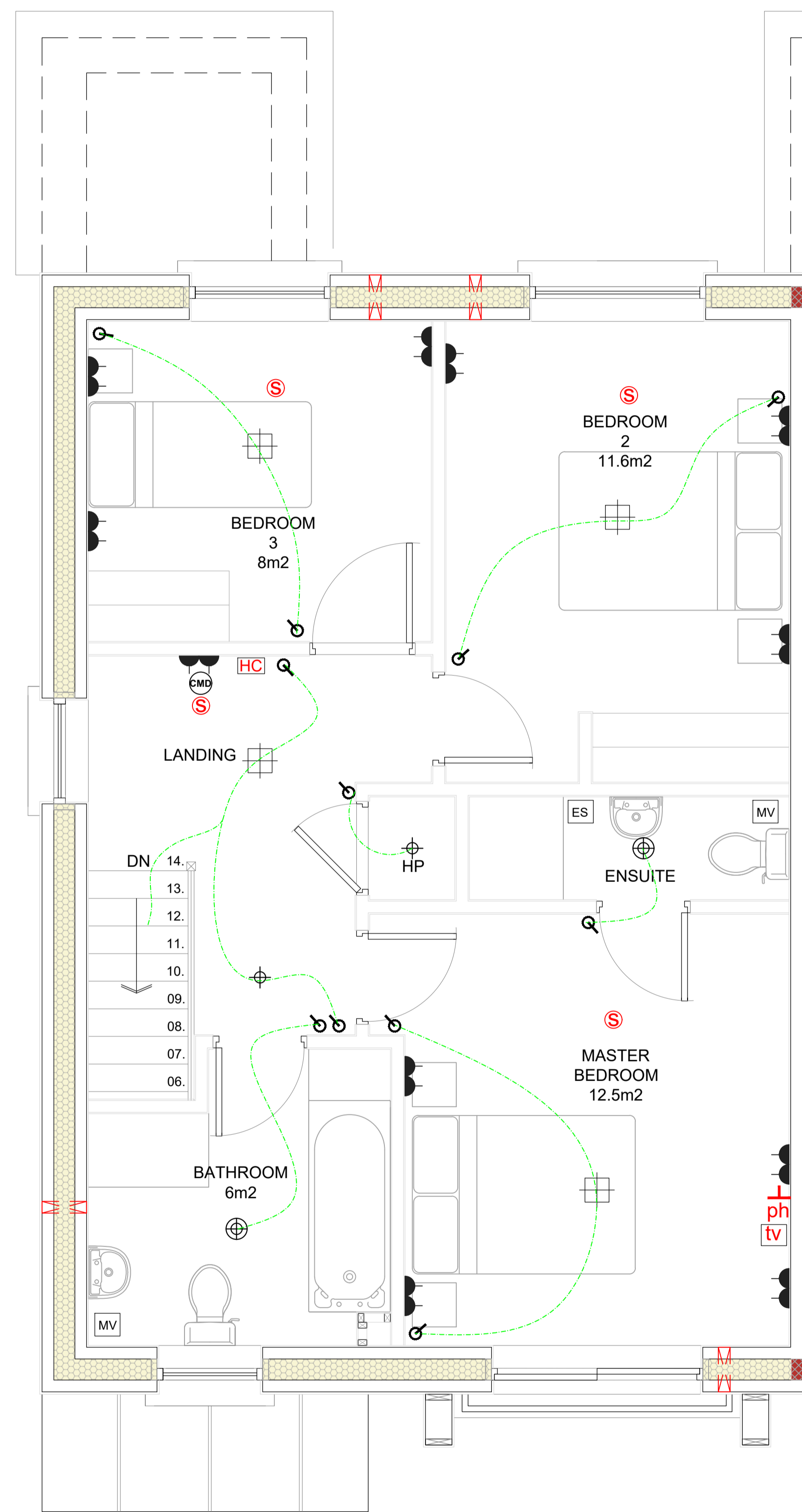
02 FIRST FLOOR PLAN SUGGESTED RCP AND SMALL POWERS NTS
